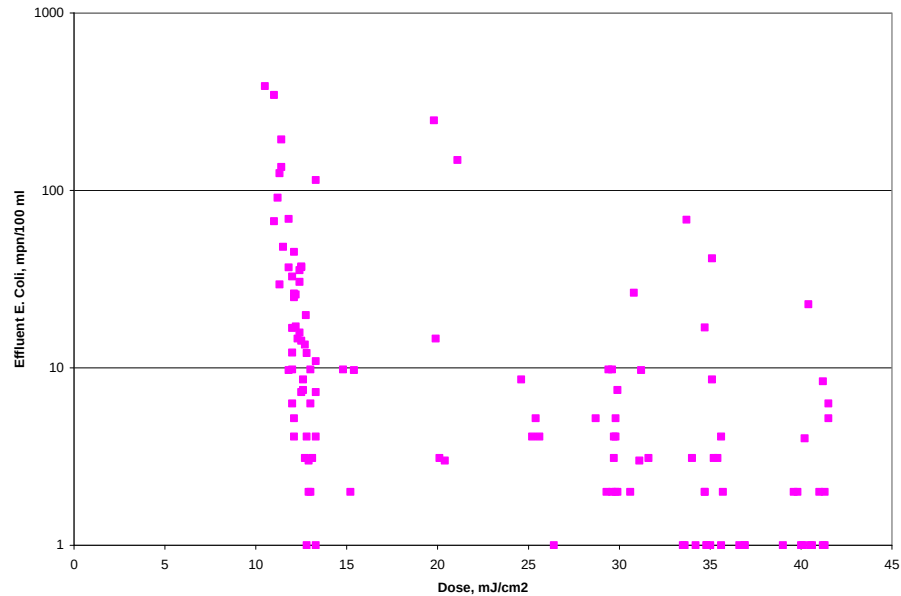
Figure 14 WEDECO Pilot Effluent E. coli Counts versus UV Dose
