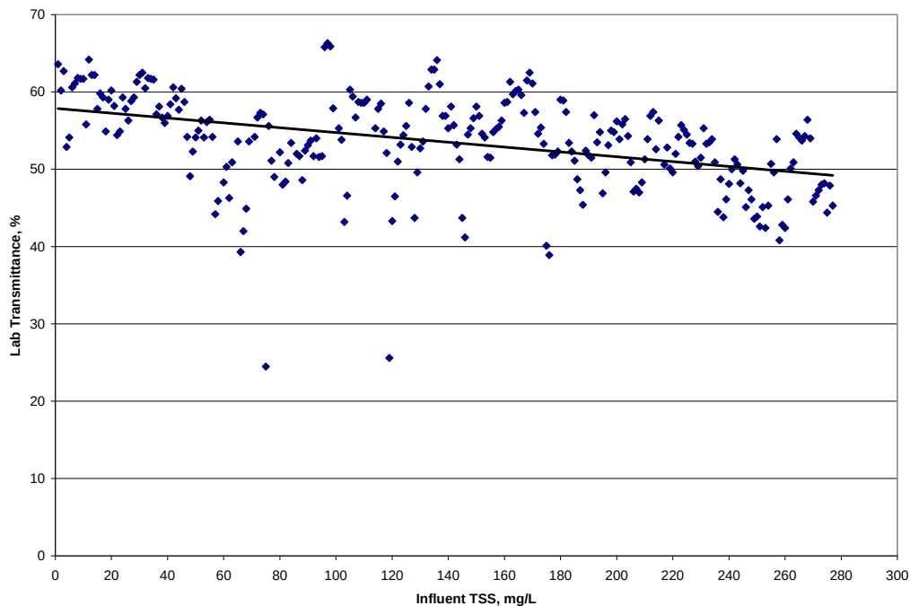
Figure 2 Trojan Pilot UV Transmittance versus Influent TSS
