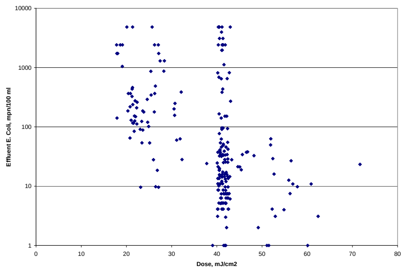
Figure 11 Trojan Pilot Effluent E. coli Counts versus UV Dose
