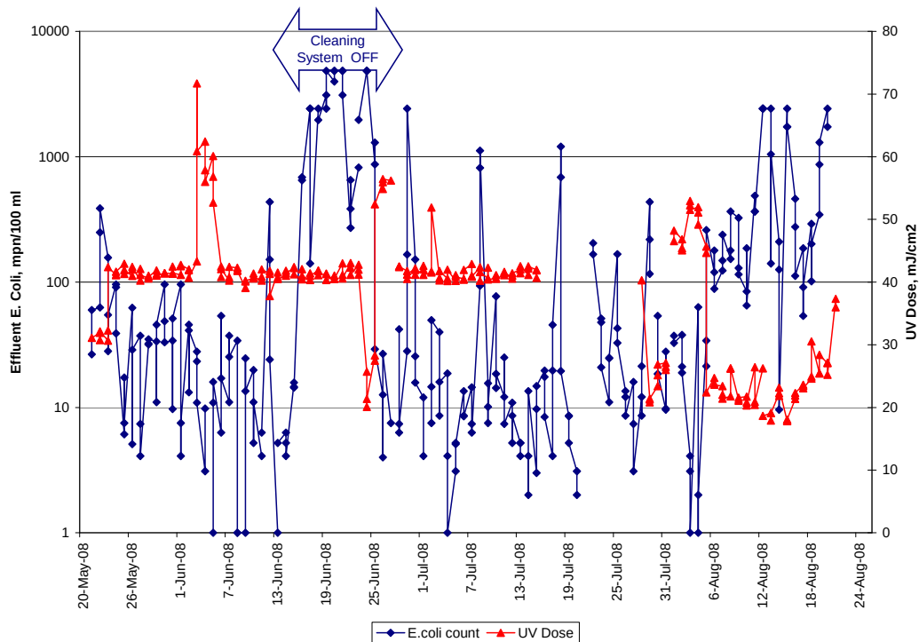
Figure 10 Trojan Pilot Effluent E. coli Counts
