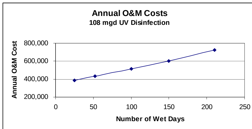
Figure 10 – Annual UV O&M Costs as a Function of the Number of Wet Days
