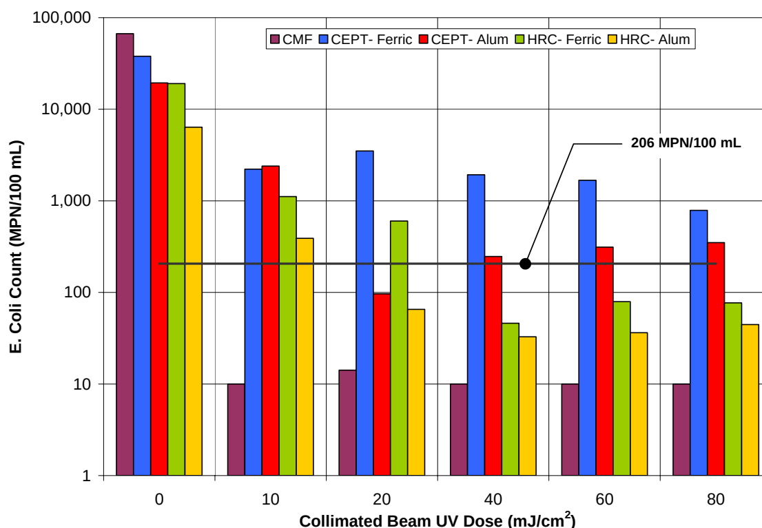
Figure 1 – Wet Weather UV Disinfection Testing Results
