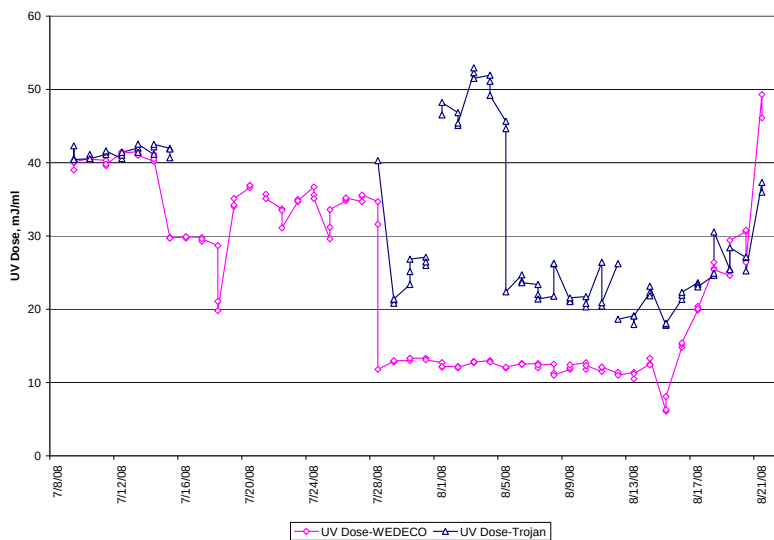
Figure 16 Pilot Comparison of Trojan and WEDECO UV Dose
