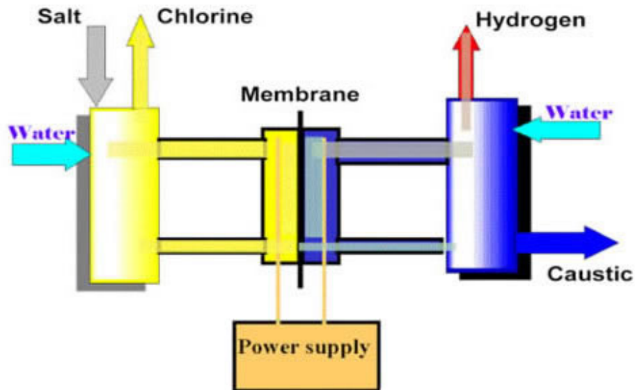
Figure 6 On-Site Sodium Hypochlorite Generation System ( http://www.electrolytictech.com )
