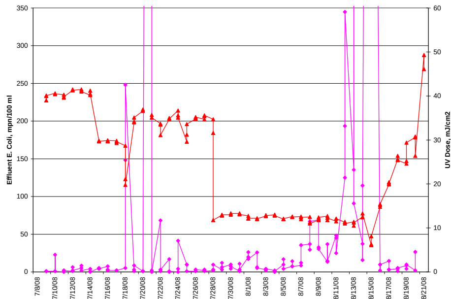
Figure 13 WEDECO Pilot Effluent E. coli Counts
