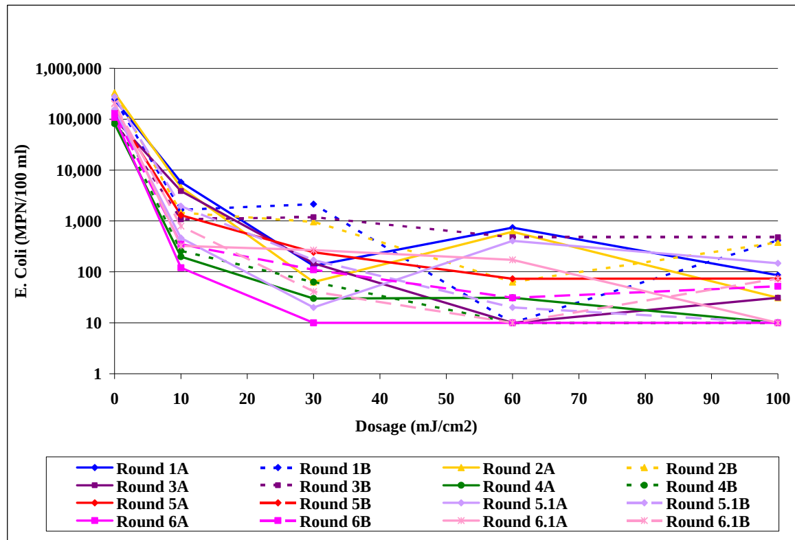
Figure 5 Blended Primary Effluent Dose Response Curve
