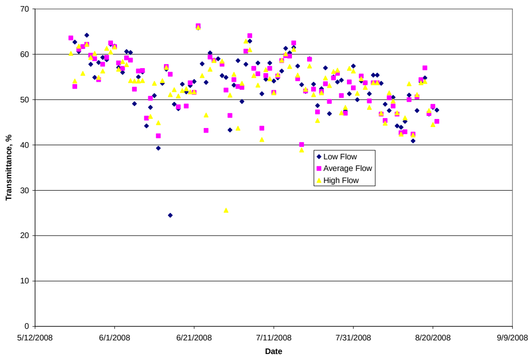
Figure 1 Effluent Transmittance Collected at Plant
