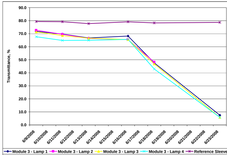
Figure 9 Results of Fouling Test
