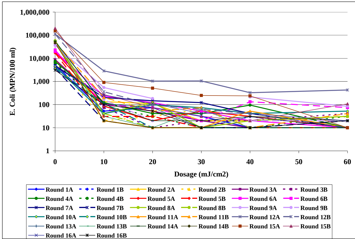
Figure 4 Secondary Effluent Dose Response Curve
