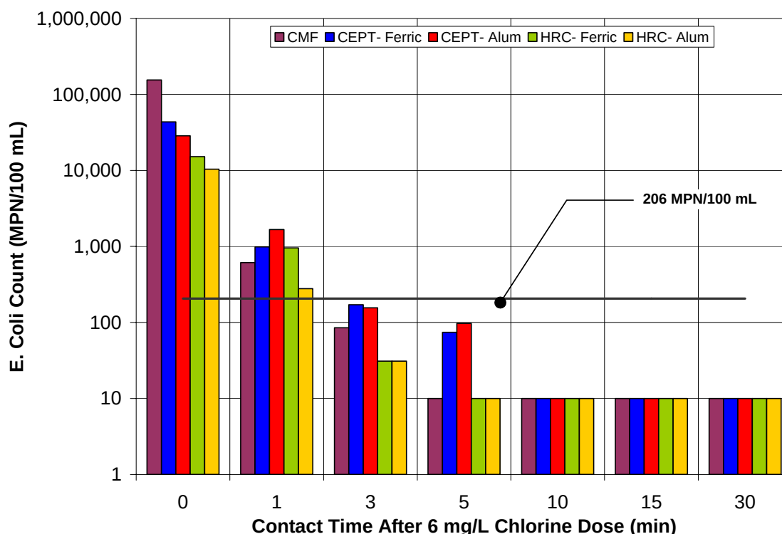
Figure 2 – Wet Weather Sodium Hypochlorite Disinfection Testing Results
