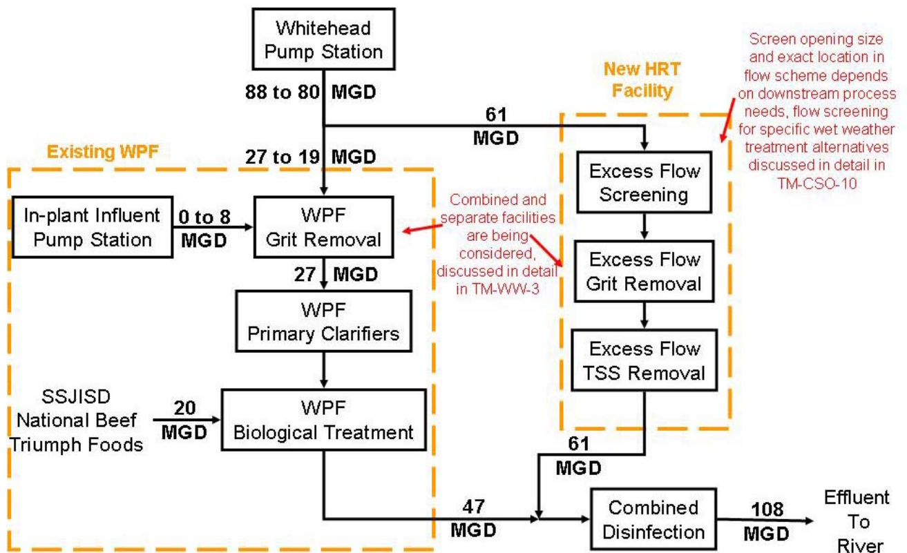
Figure 3 – Combined Disinfection Facility Alternative
