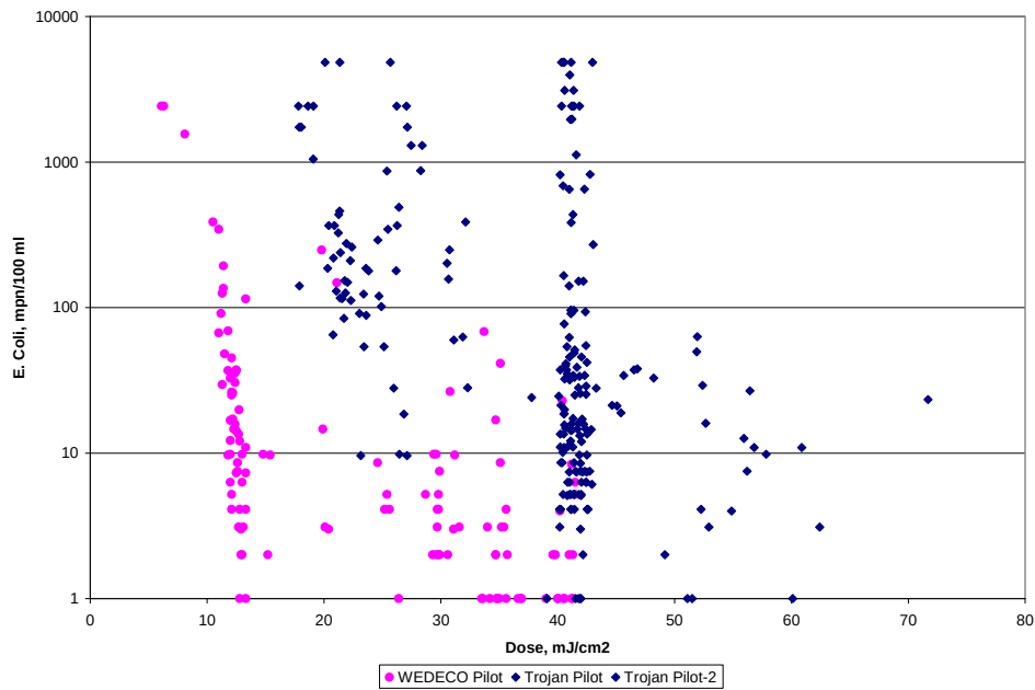
Figure 17 Pilot Comparison of Effluent E. coli Count versus UV Dose
