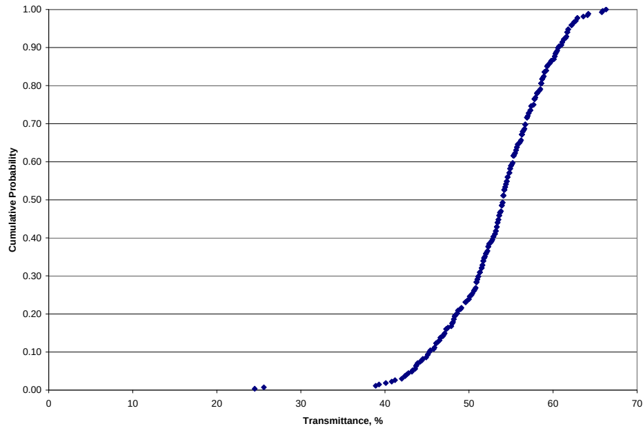
Figure 3 Pilot UV Transmittance Cumulative Distribution
