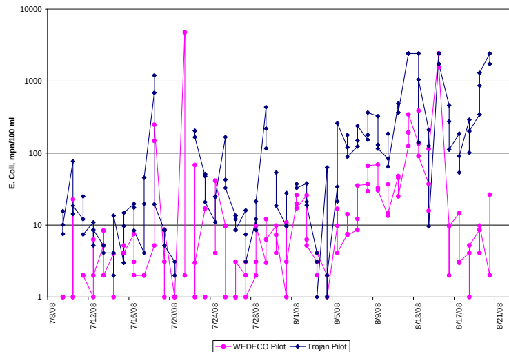
Figure 15 Pilot Comparison of Trojan and WEDECO Effluent E. coli Counts
